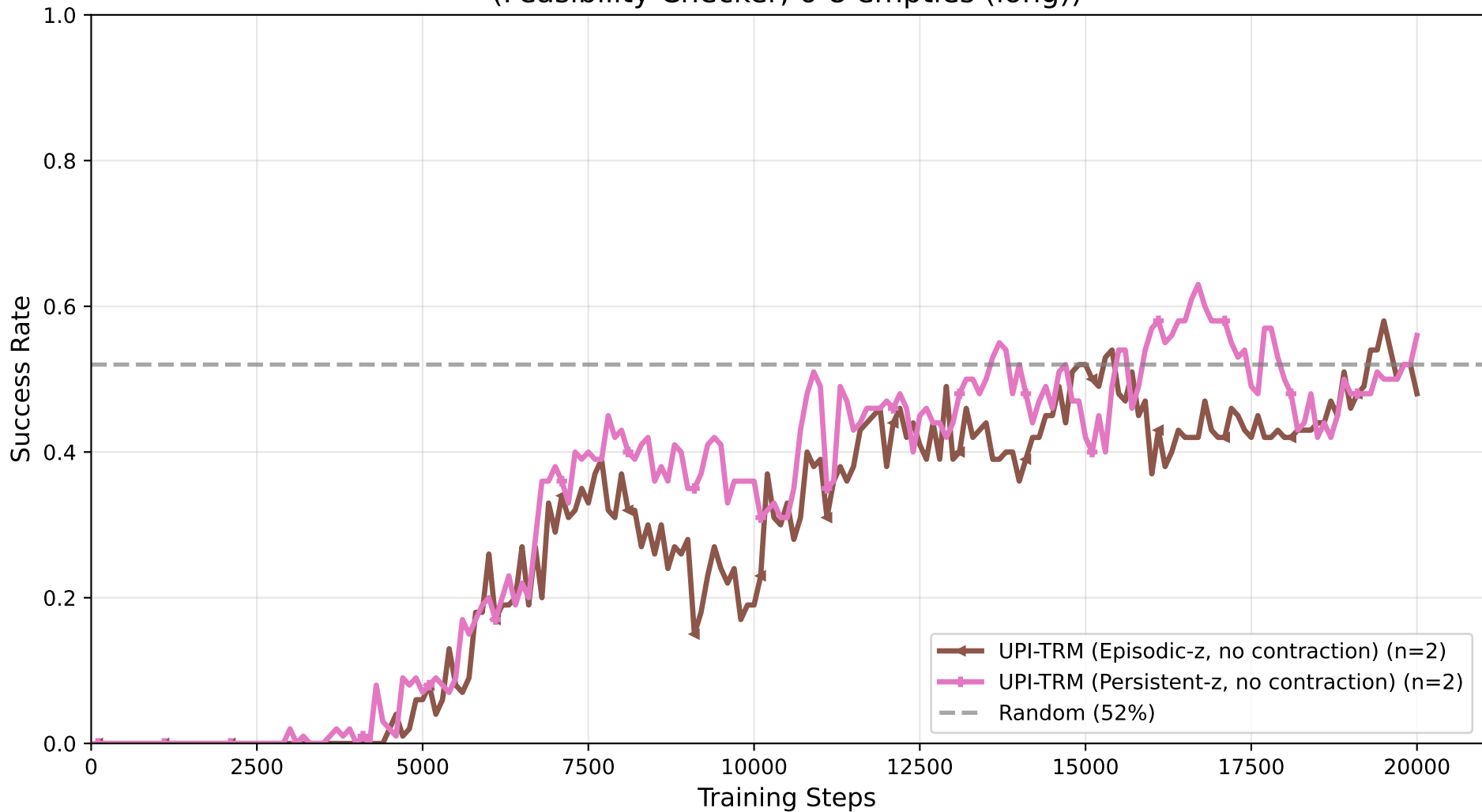
4×4 Sudoku: Ablation Study (Feasibility Checker, 6-8 empties (long))
