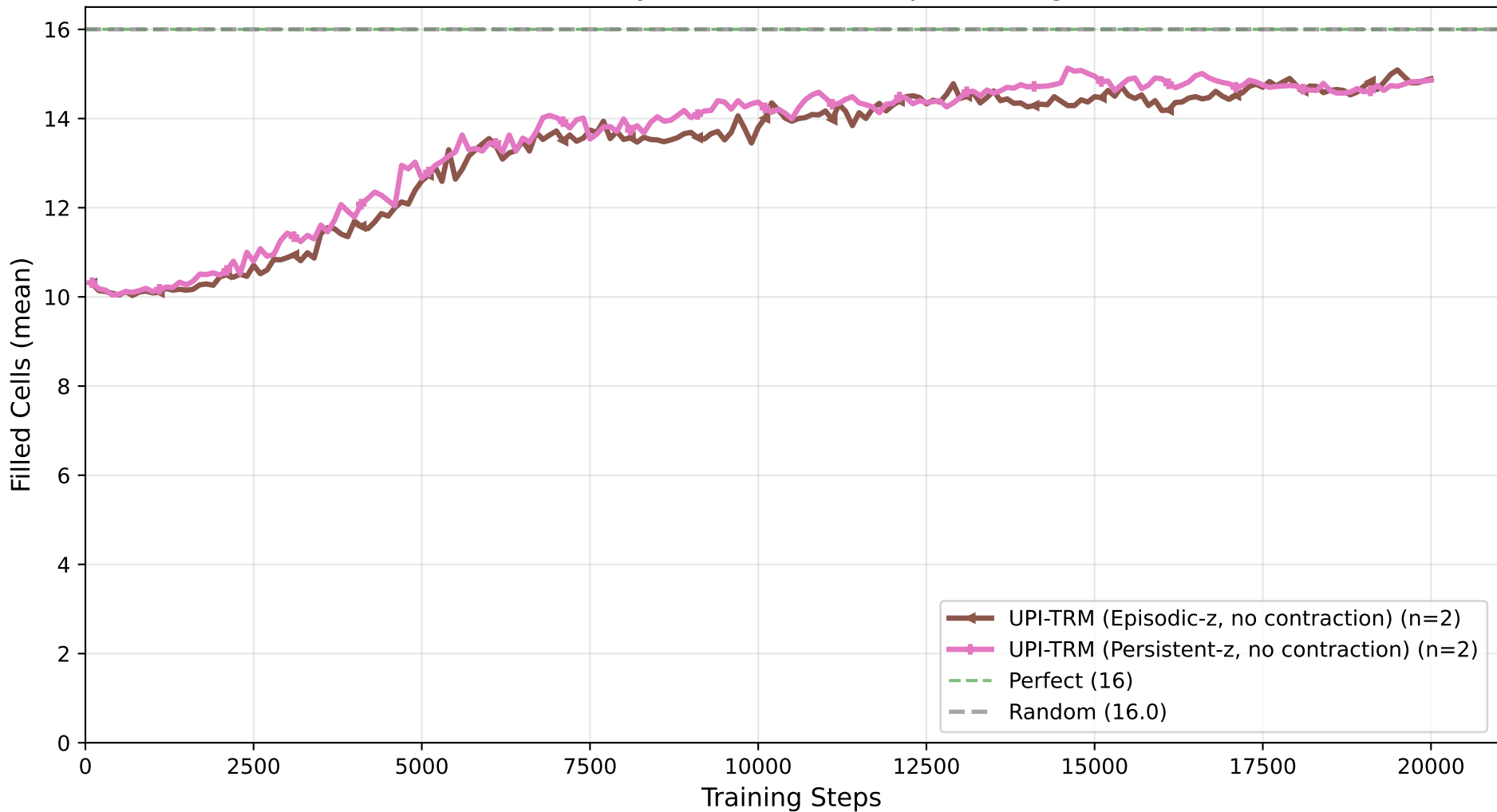
4×4 Sudoku: Filled Cells vs Training Steps (Feasibility Checker, 6-8 empties (long))
