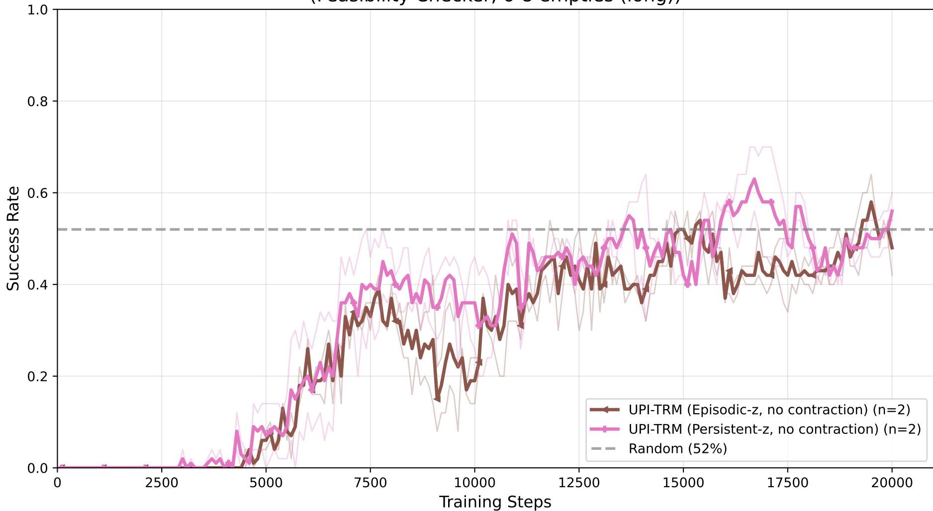
4×4 Sudoku: Success Rate vs Training Steps (Feasibility Checker, 6-8 empties (long))
