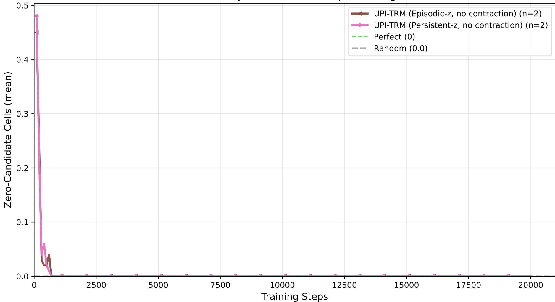
4×4 Sudoku: Dead-End Cells vs Training Steps (Feasibility Checker, 6-8 empties (long))
