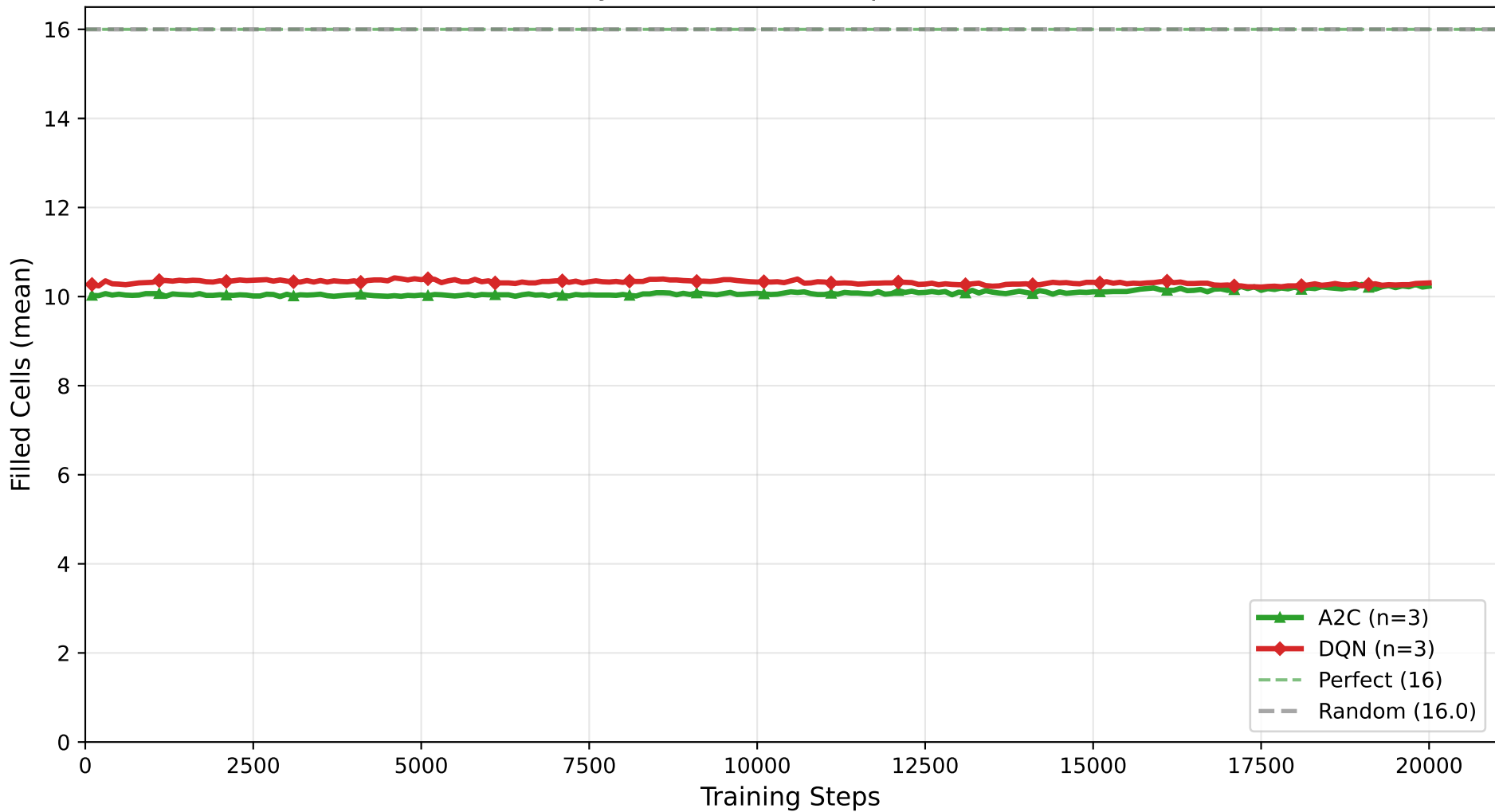
4×4 Sudoku: Filled Cells vs Training Steps (Feasibility Checker, 6-8 empties (baselines))
