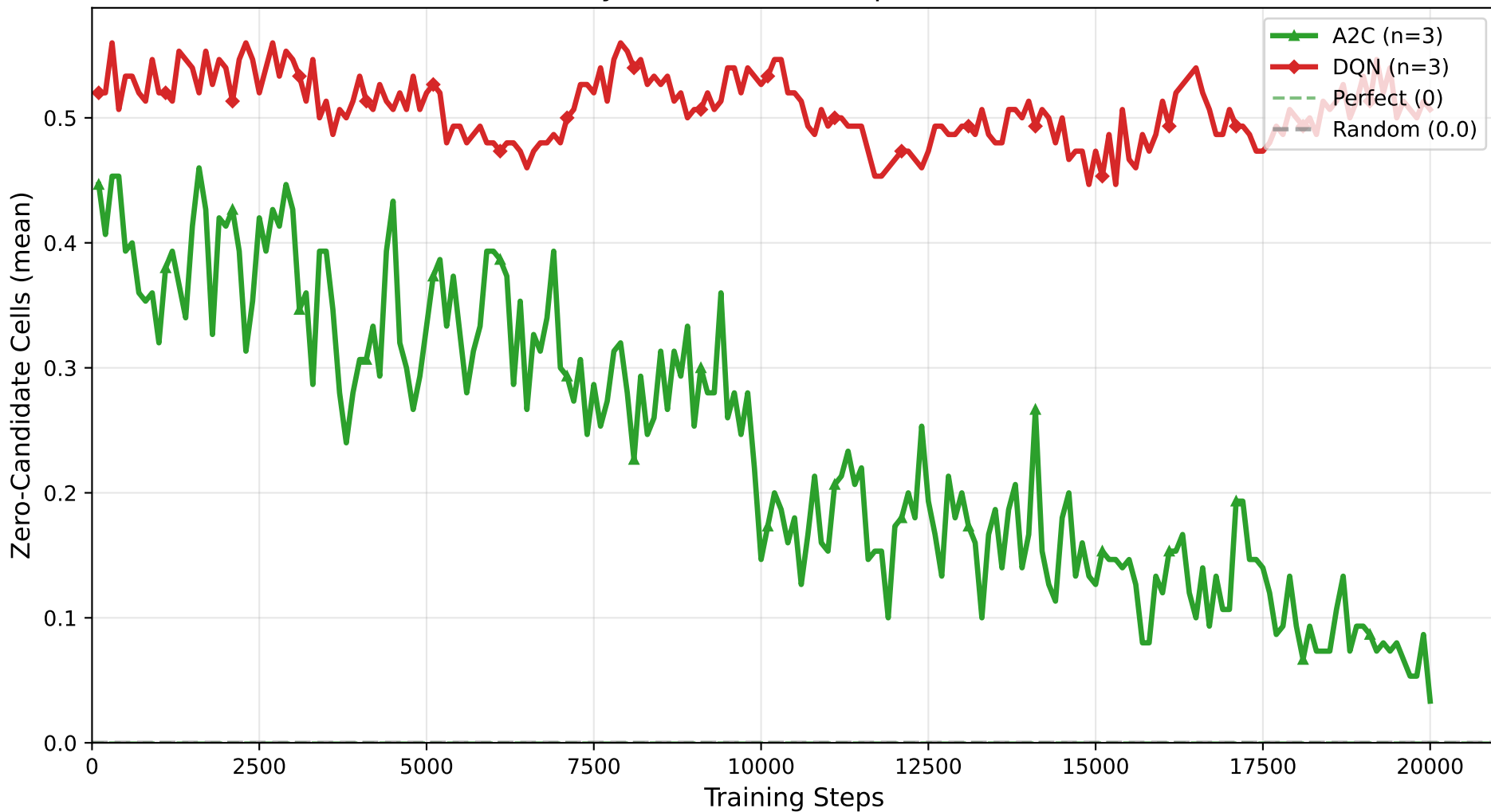
4x4 Sudoku: Dead-End Cells vs Training Steps (Feasibility Checker, 6-8 empties (baselines))
