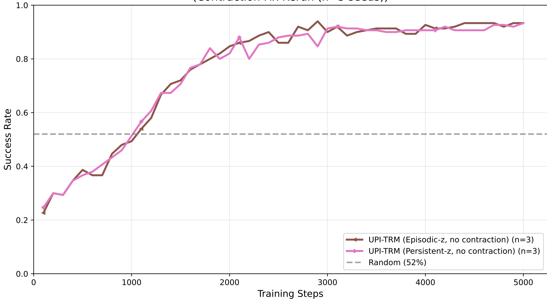
4×4 Sudoku: Ablation Study (Contraction Fix Rerun (n=3 seeds))
