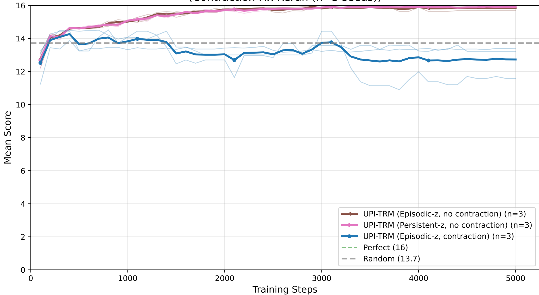
4×4 Sudoku: Mean Score vs Training Steps (Contraction Fix Rerun (n=3 seeds))
