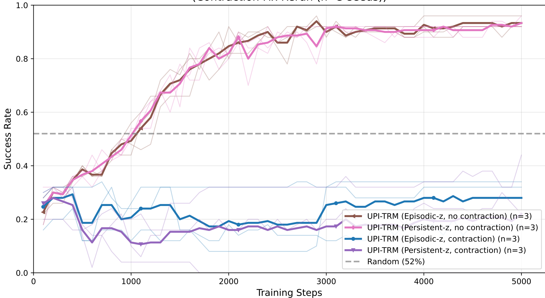
4x4 Sudoku: Success Rate vs Training Steps (Contraction Fix Rerun (n=3 seeds))
