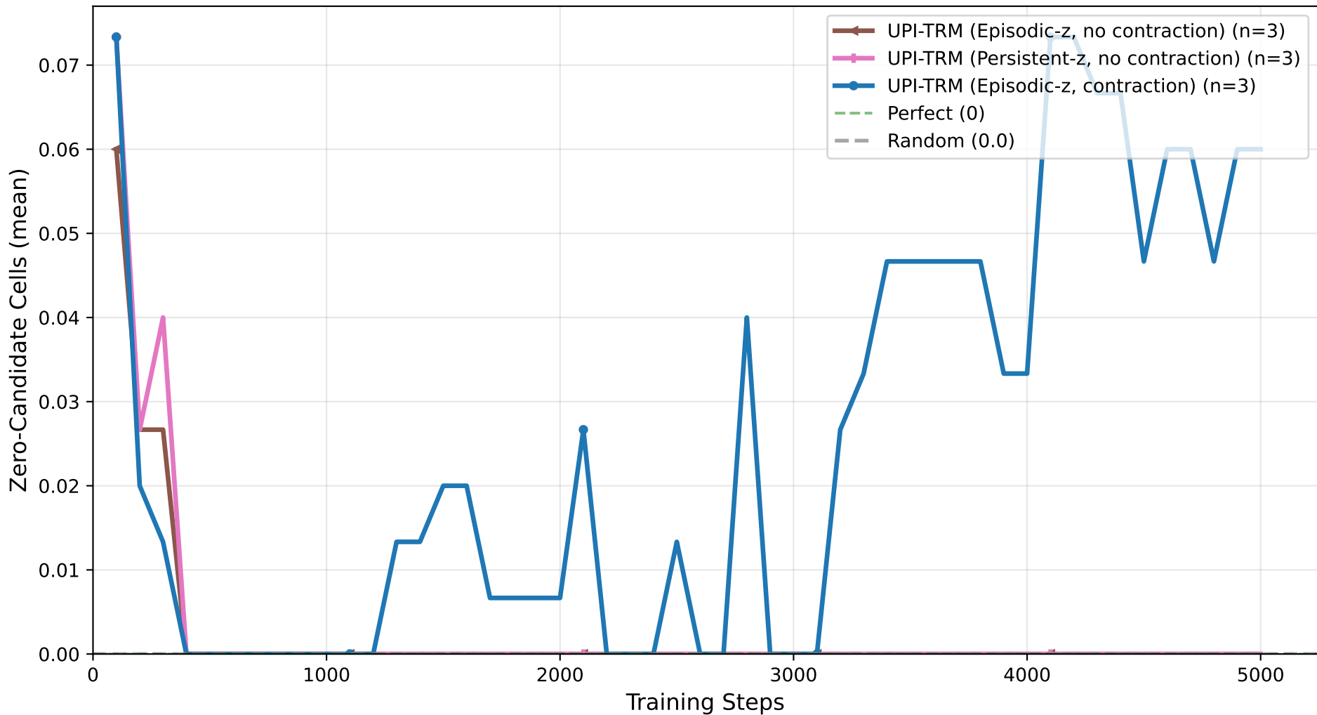
4×4 Sudoku: Dead-End Cells vs Training Steps (Contraction Fix Rerun (n=3 seeds))
