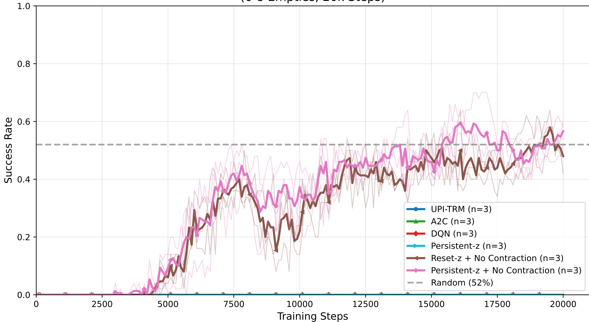
4×4 Sudoku: Success Rate vs Training Steps (6-8 Empties, 20k Steps)
