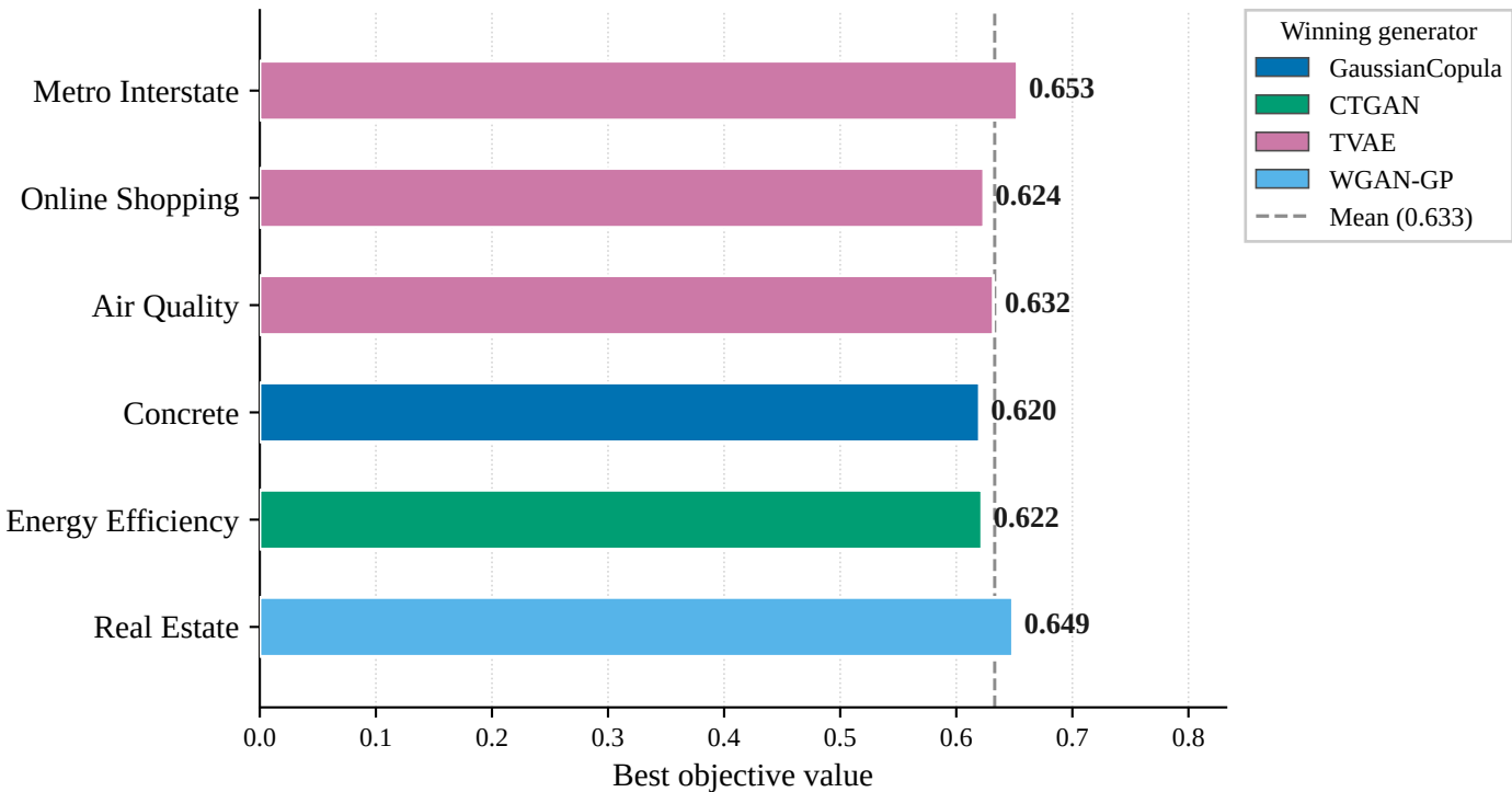
Best Optuna objective by regression dataset
