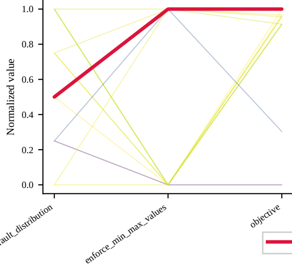
Concrete — GaussianCopula best trial 10 (obj=0.620)
