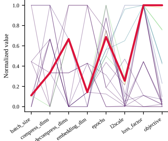
Concrete — GaussianCopula best trial 10 (obj=0.620)
