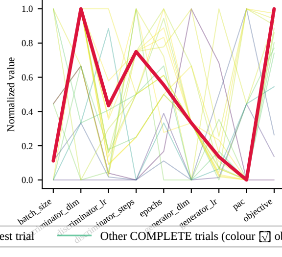
Energy Efficiency — CTGAN best trial 13 (obj=0.622)
