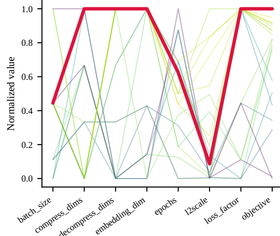
Energy Efficiency — CTGAN best trial 13 (obj=0.622)
