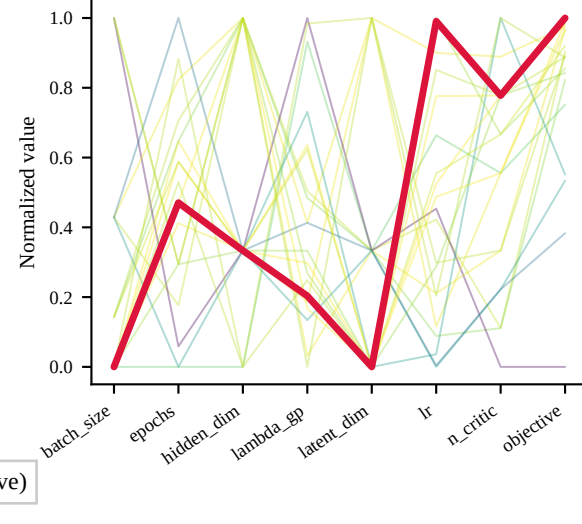
Real Estate — WGAN-GP best trial 13 (obj=0.649)
