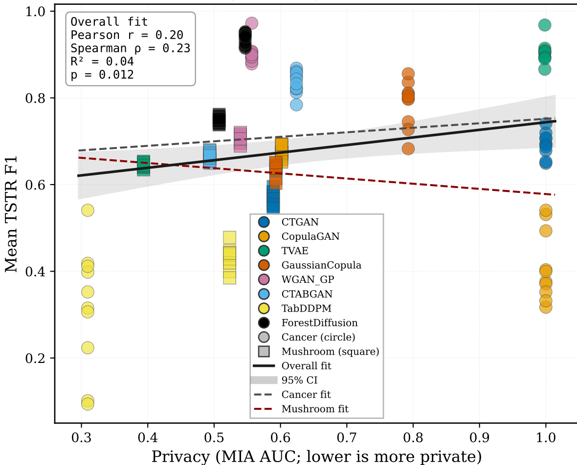
Privacy vs Utility (F1, MIA AUC)
