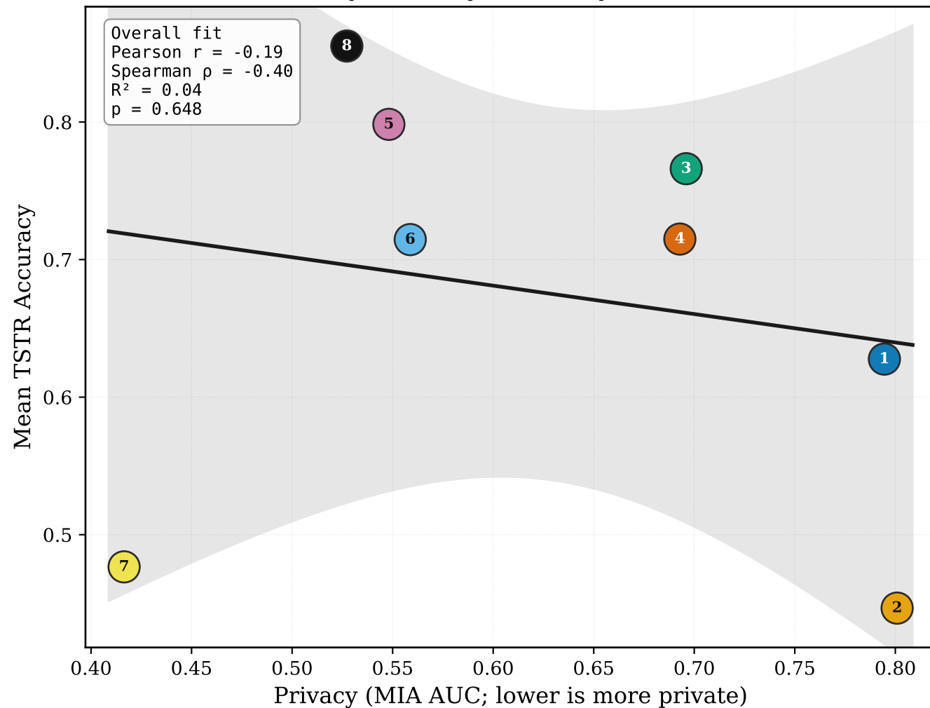
Privacy vs Utility (Accuracy, MIA AUC)
