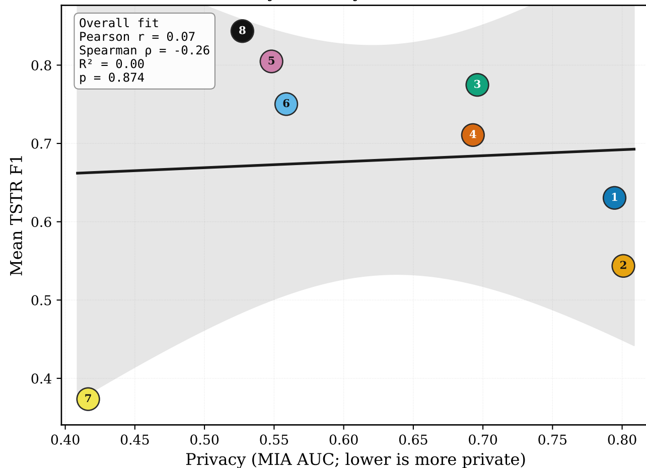
Privacy vs Utility (F1, MIA AUC)
