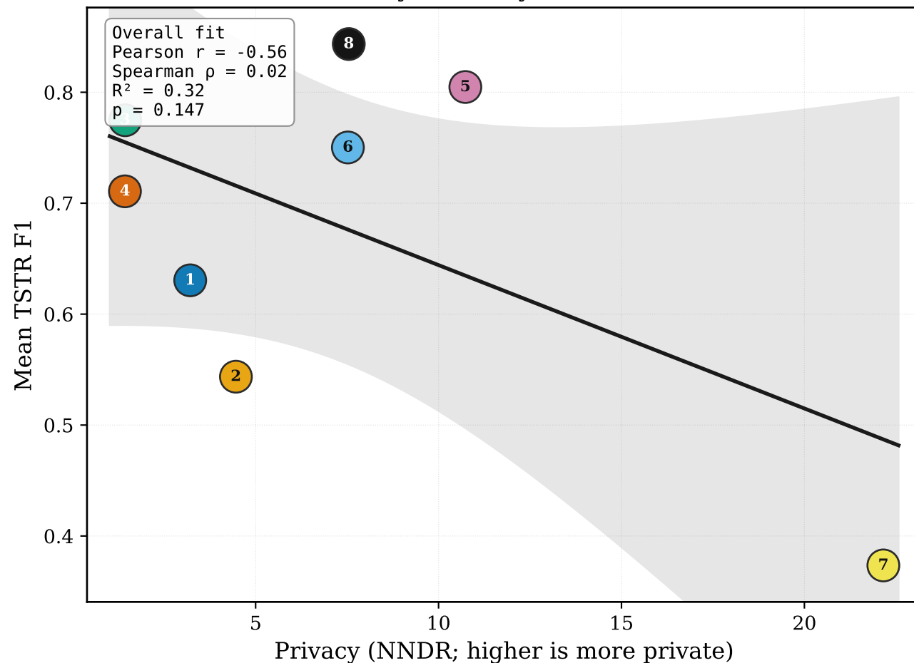
Privacy vs Utility (F1, NNDR)
