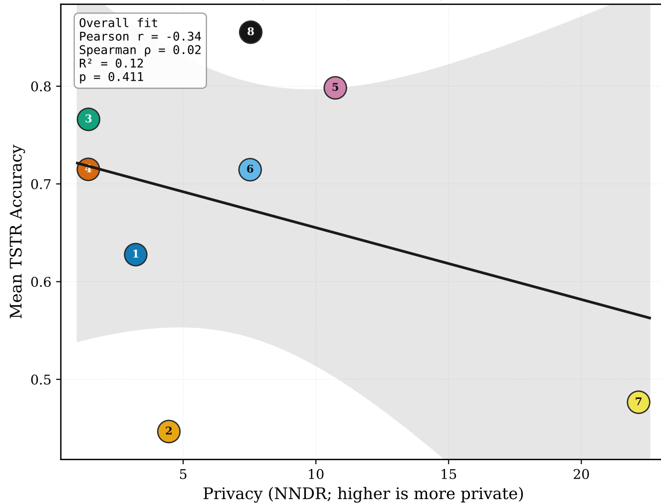
Privacy vs Utility (Accuracy, NNDR)
