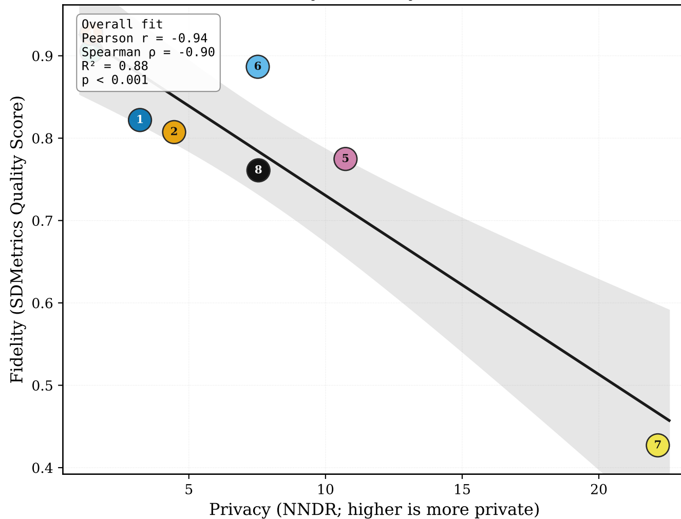
Fidelity vs Privacy (NNDR)
