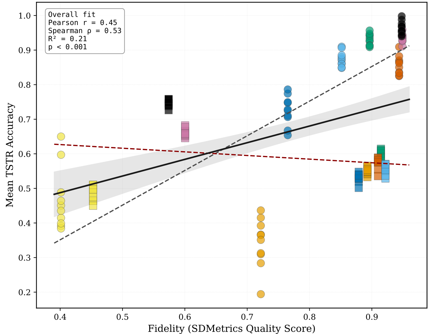
Supplementary: Fidelity vs Utility (Accuracy; seed-level)
