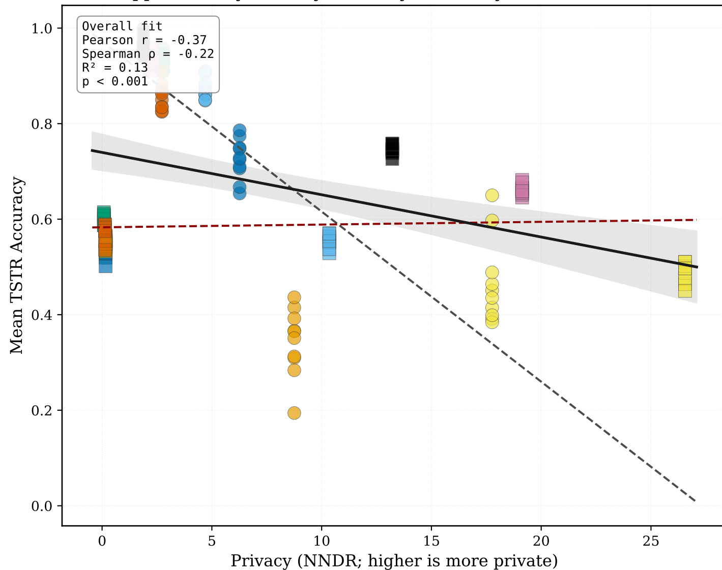
Supplementary: Privacy vs Utility (Accuracy, NNDR; seed-level)
