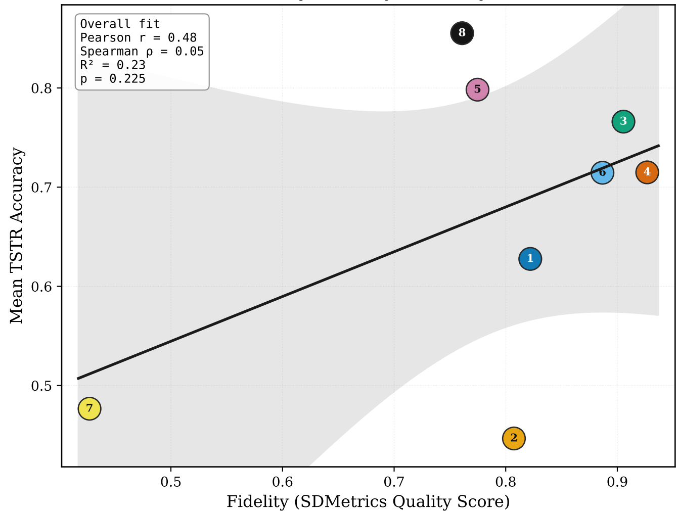
Fidelity vs Utility (Accuracy)
