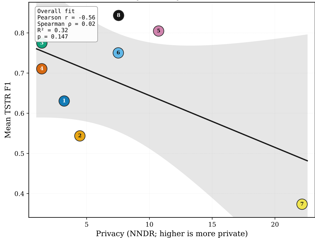
Privacy vs Utility (F1, NNDR)
