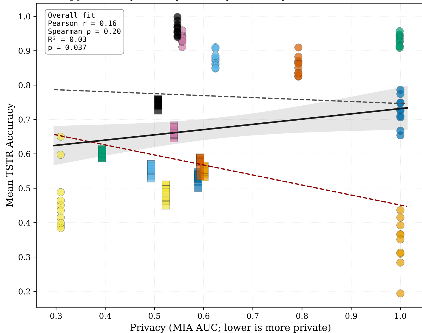
Supplementary: Privacy vs Utility (Accuracy, MIA AUC; seed-level)
