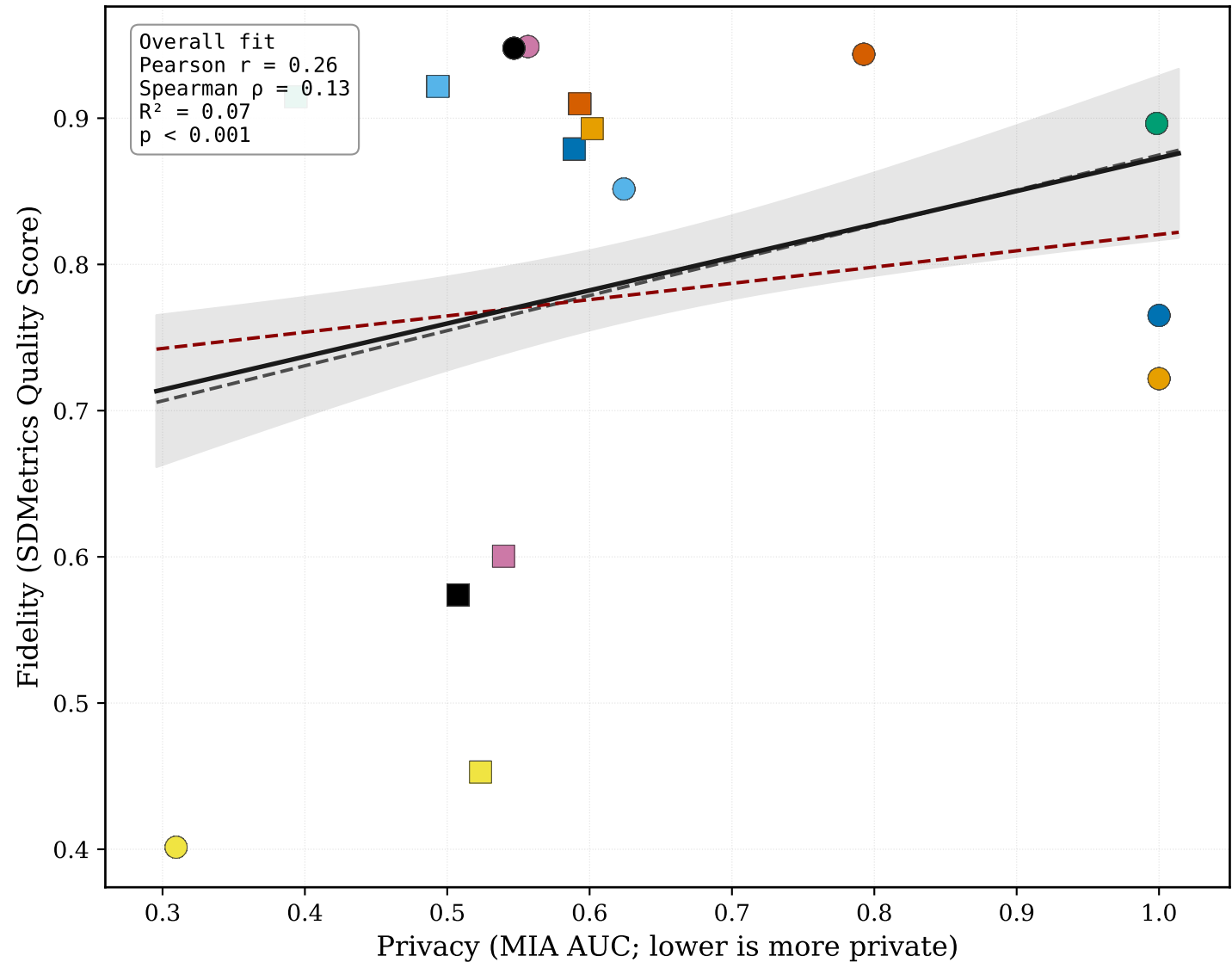
Supplementary: Fidelity vs Privacy (MIA AUC; seed-level)
