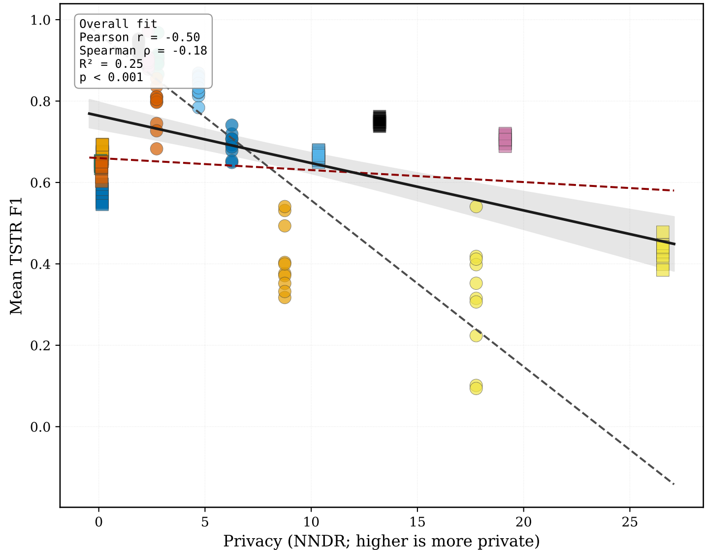
Supplementary: Privacy vs Utility (F1, NNDR; seed-level)
