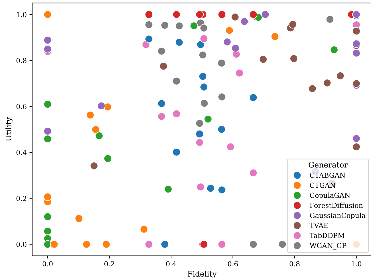
Fidelity vs Utility
