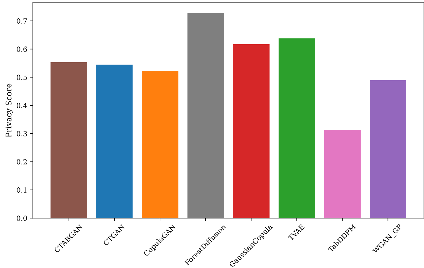
Figure 8: Privacy by Generator (Leakage=0% baseline)
