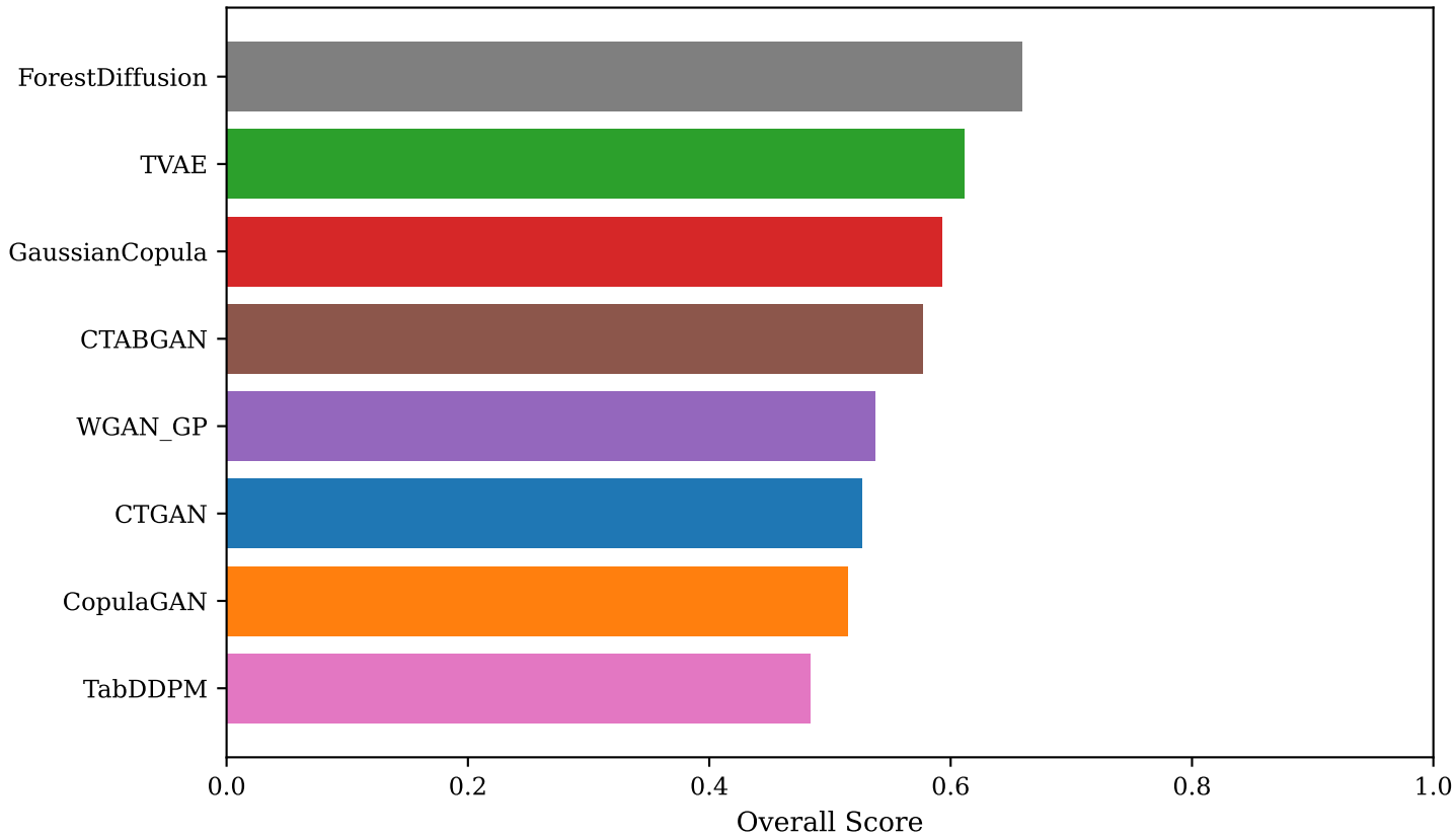
Figure 6: Overall Generator Ranking
