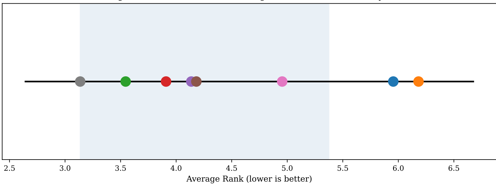
Figure 13: Critical Difference Diagram (Friedman + Nemenyi)
