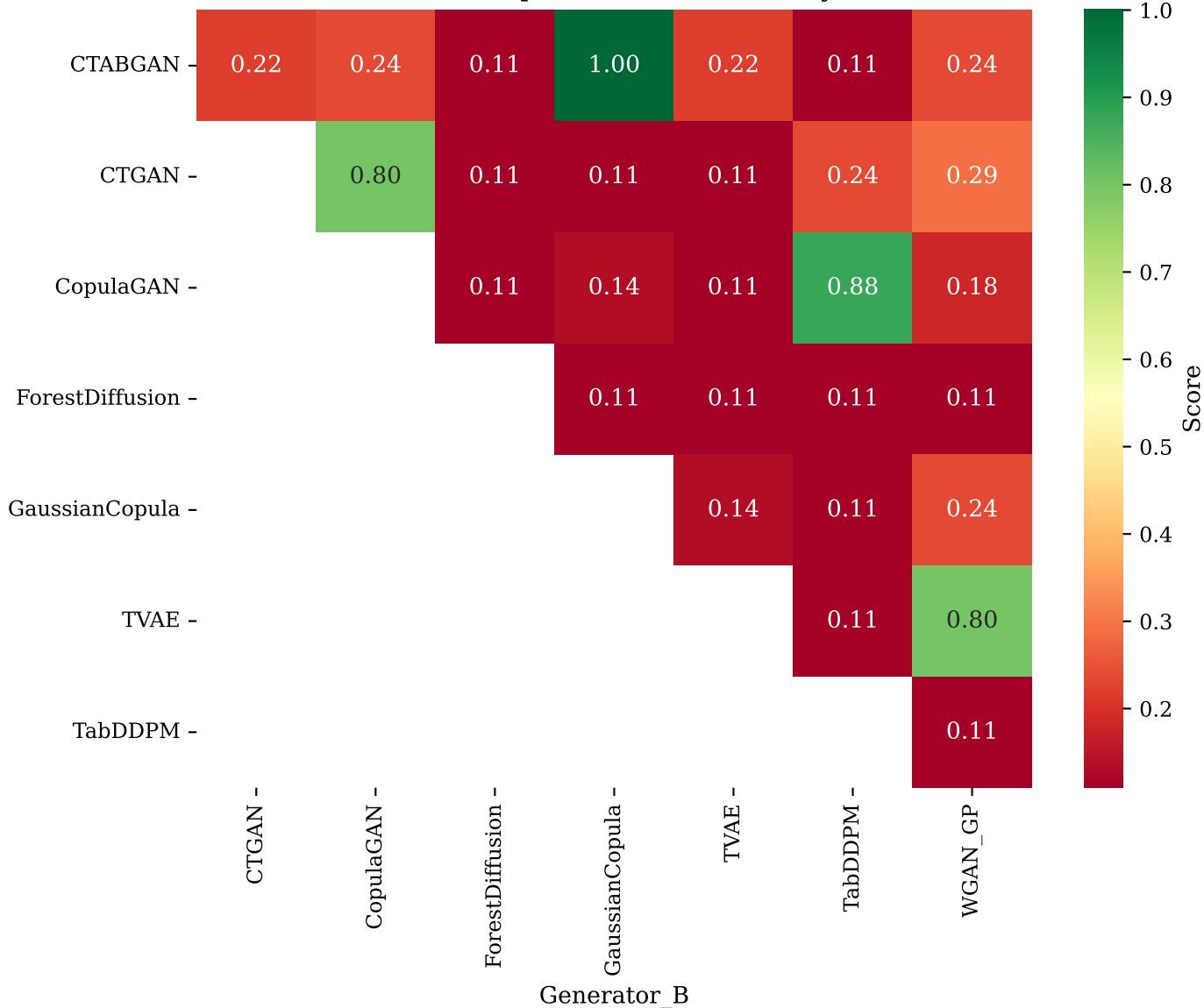
Wilcoxon p-values (BH): Accuracy
