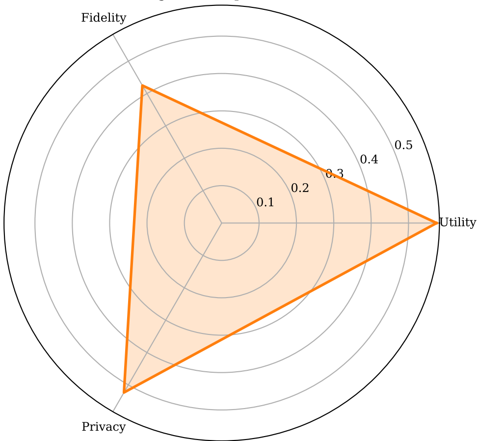
Figure 5: CopulaGAN
