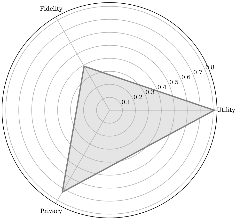
Figure 5: ForestDiffusion
