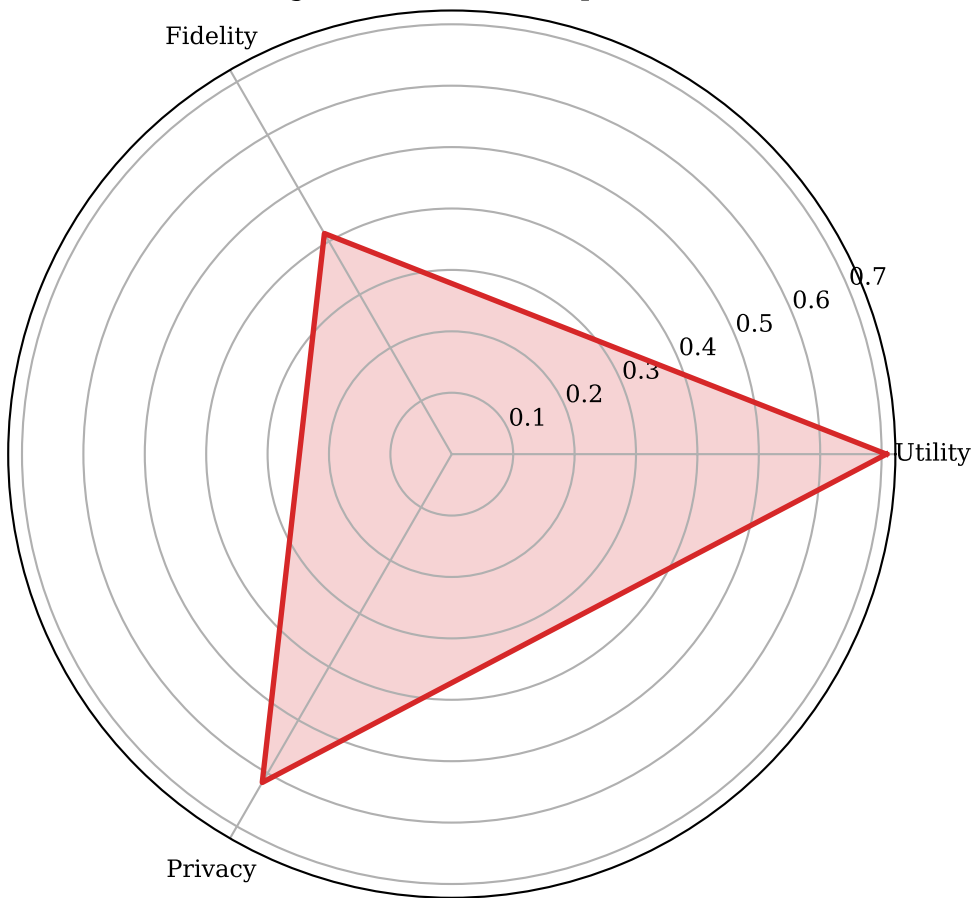
Figure 5: GaussianCopula
