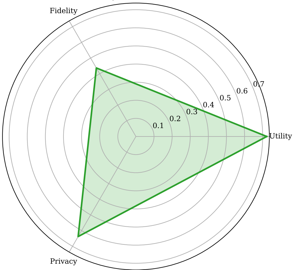
Figure 5: TVAE
