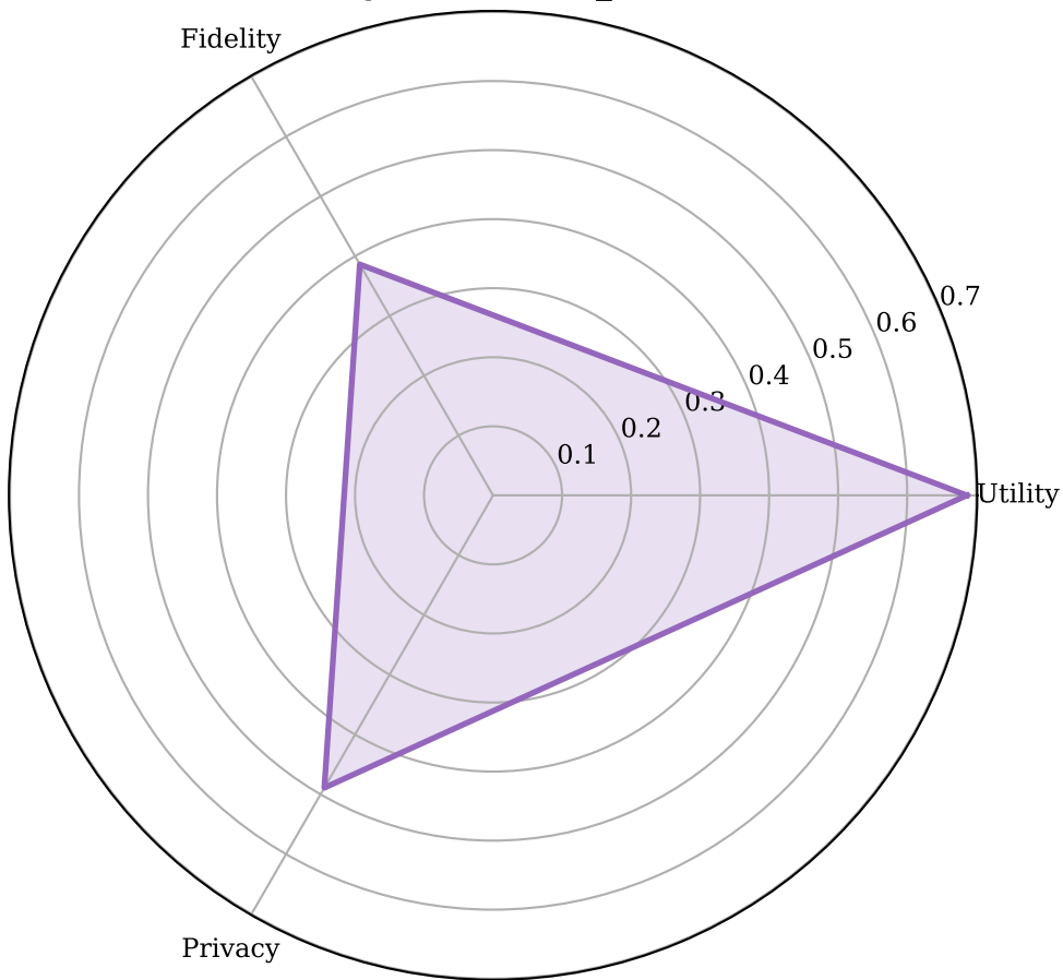
Figure 5: WGAN_GP
