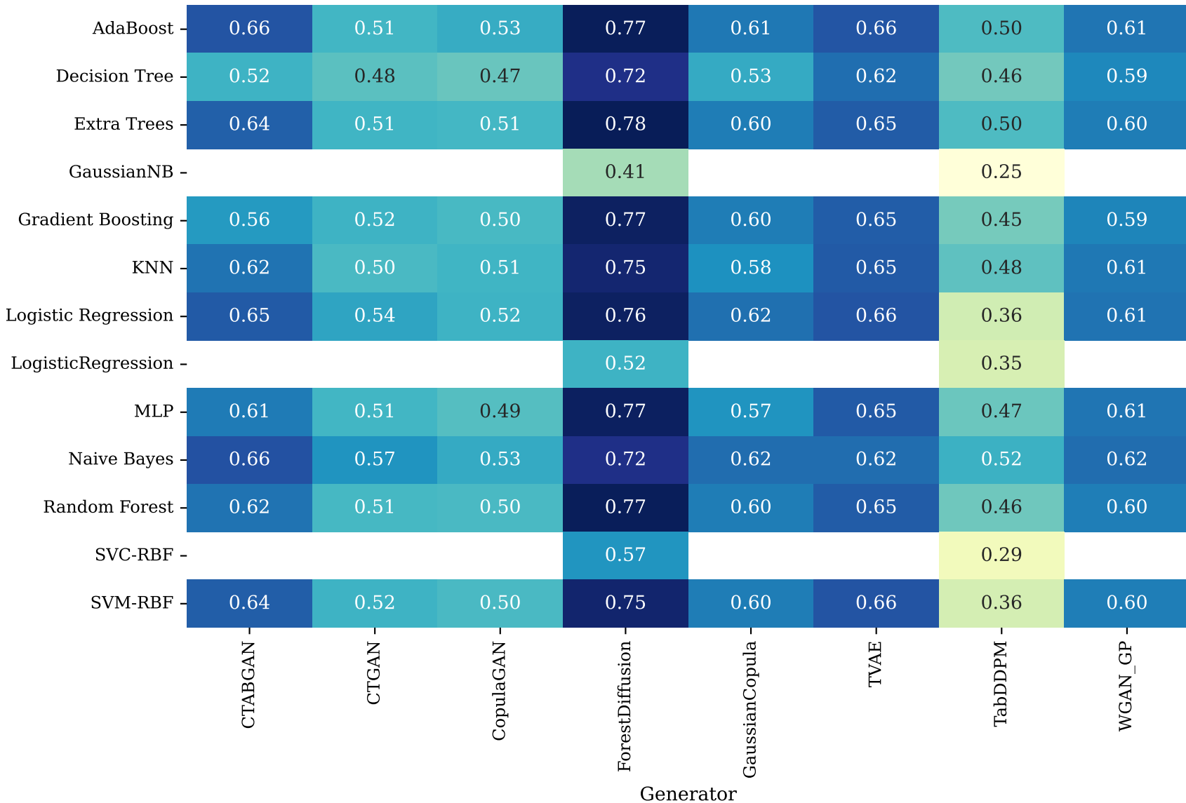
Figure 10: F1 by Classifier × Generator
