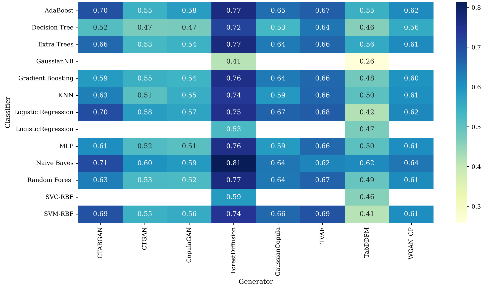
Figure 10: Recall by Classifier × Generator
