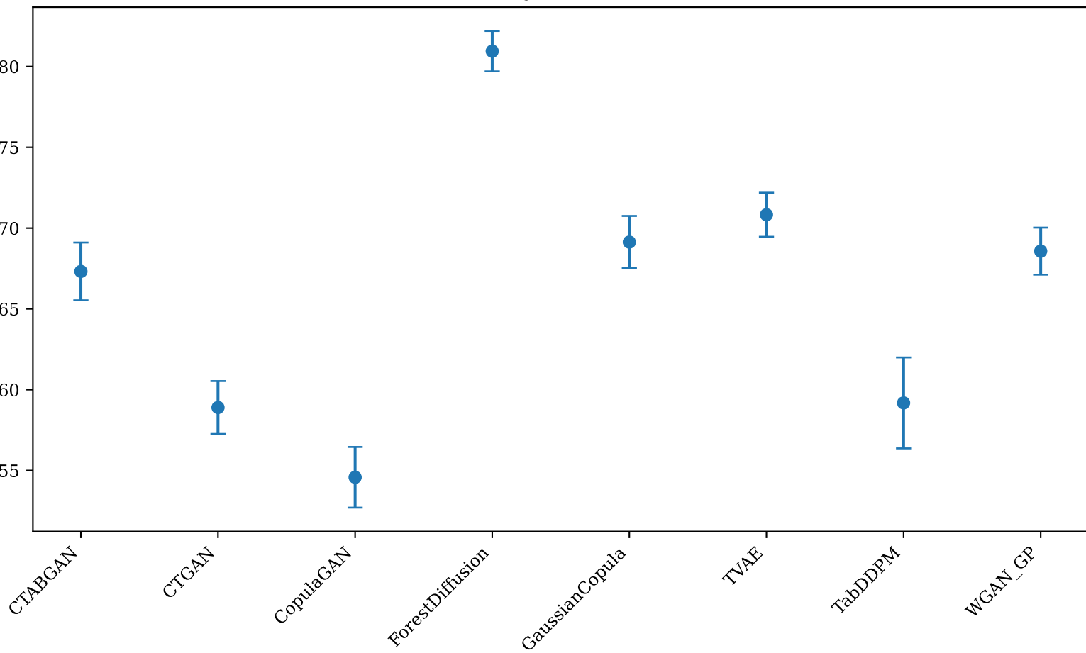
Accuracy TSTR 95% CI
