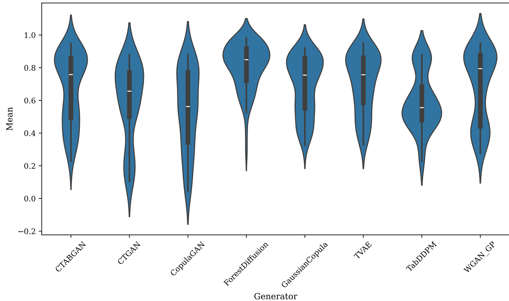
Accuracy TSTR Violin
