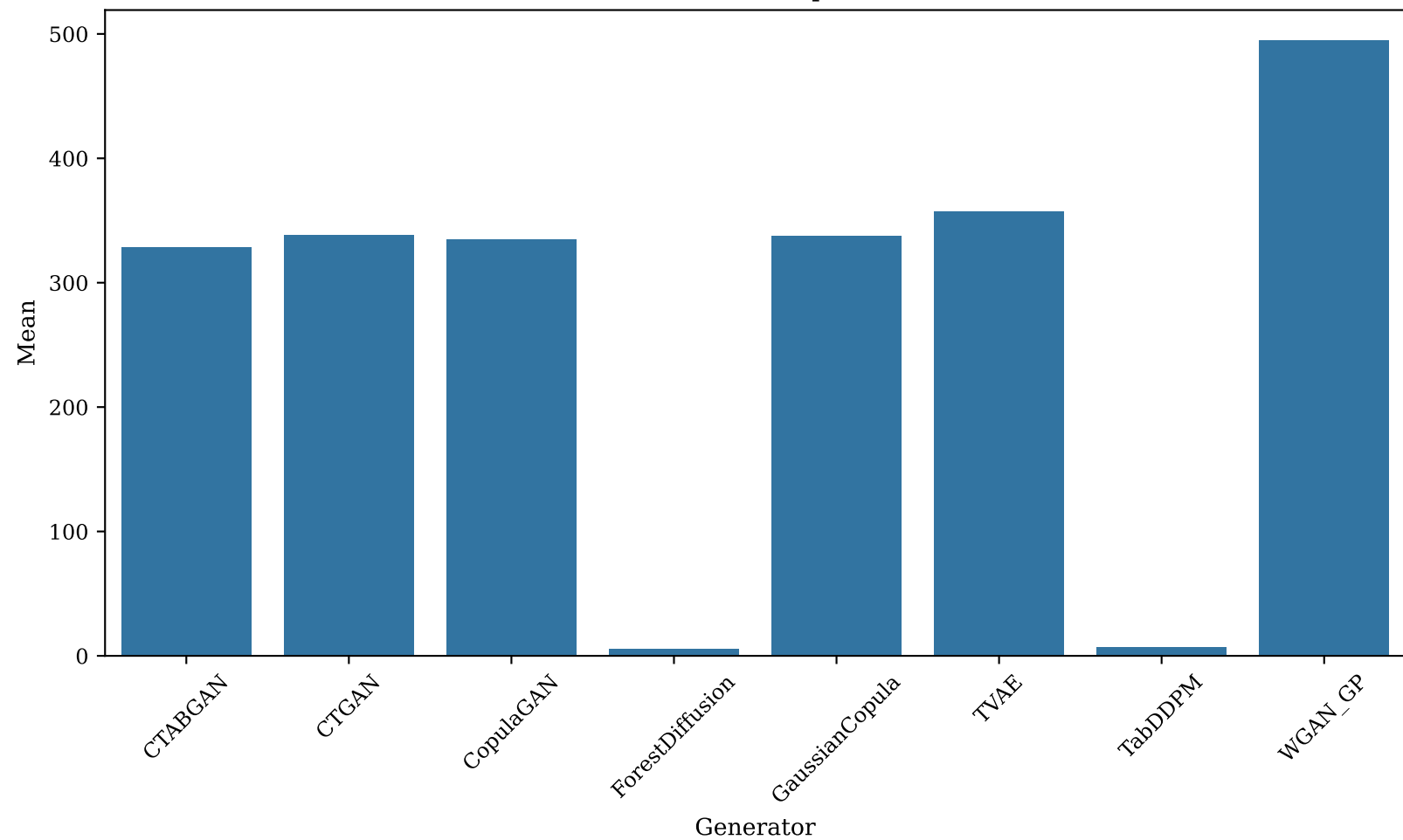
MAE TSTR Comparison
