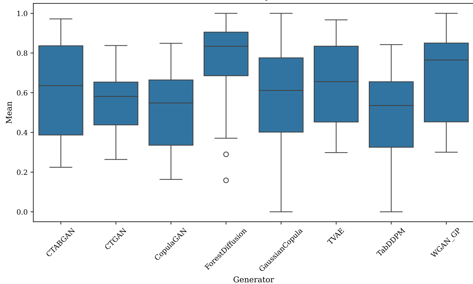
Precision TSTR by Generator
