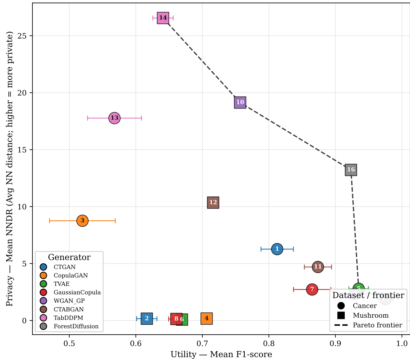
Utility vs Privacy (Supplementary — best classifier)
