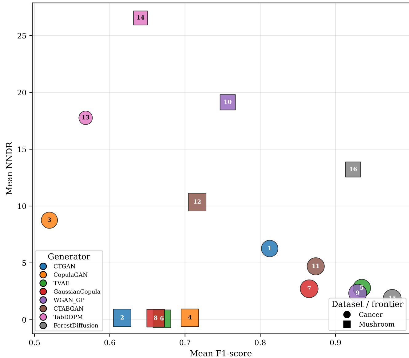
Bubble Trade-off (size = Quality) (Supplementary — best classifier)
