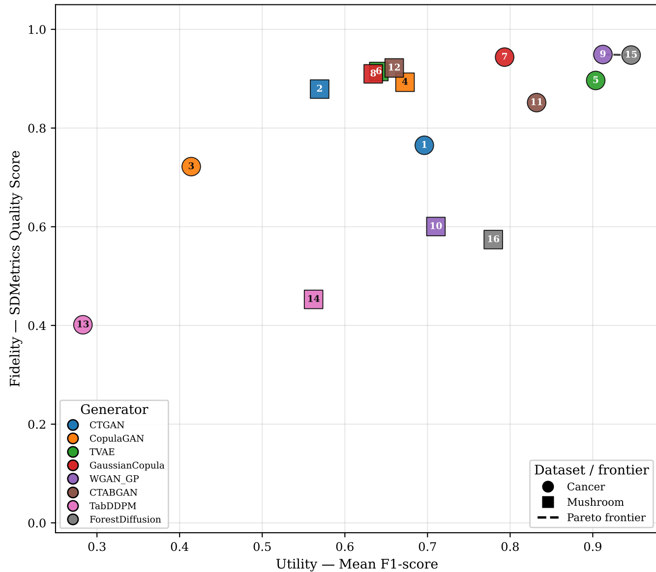
Utility vs Fidelity (Primary — classifier-independent)
