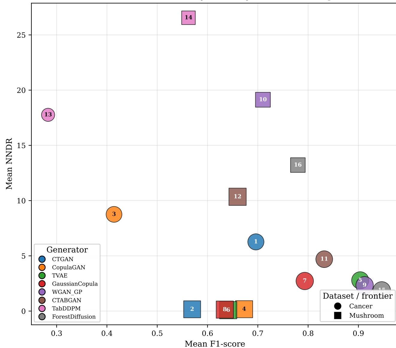
Bubble Trade-off (size = Quality) (Primary — classifier-independent)
