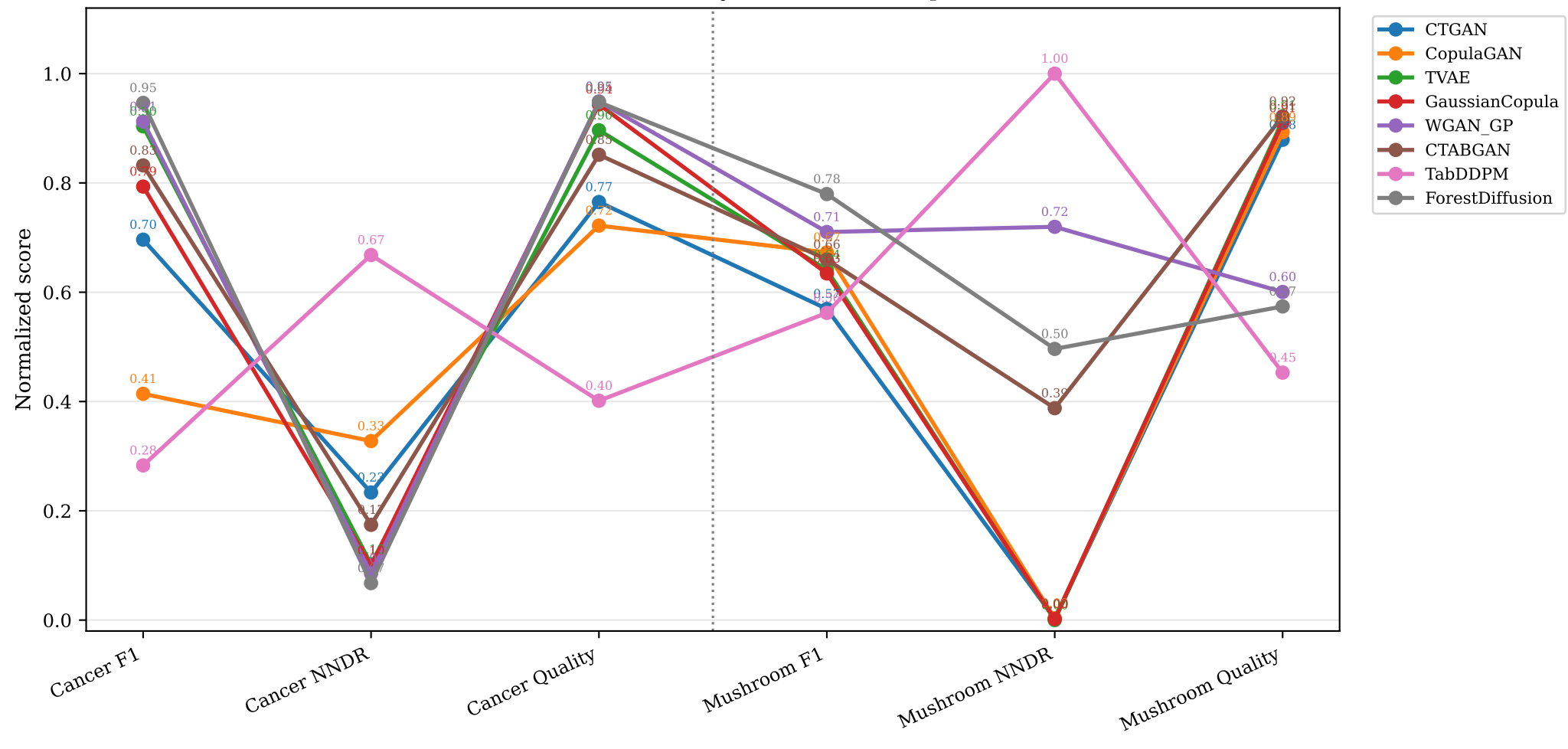
Parallel Coordinates (Primary — classifier-independent)
