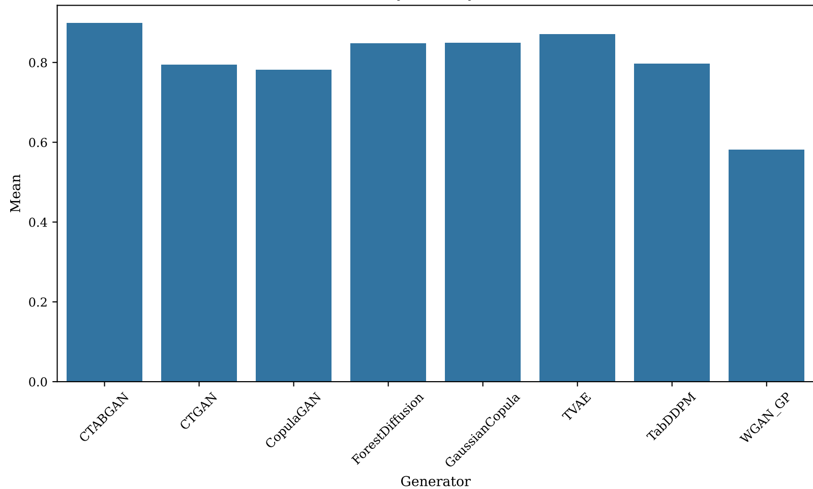
SDV Quality Score by Generator
