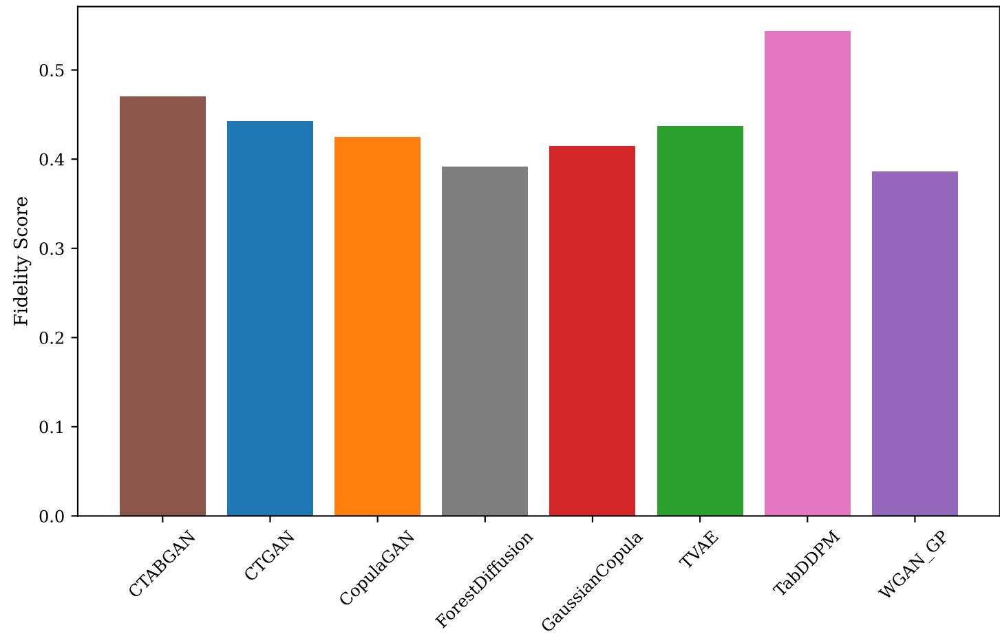
Figure 8: Fidelity by Generator (Leakage=0% baseline)
