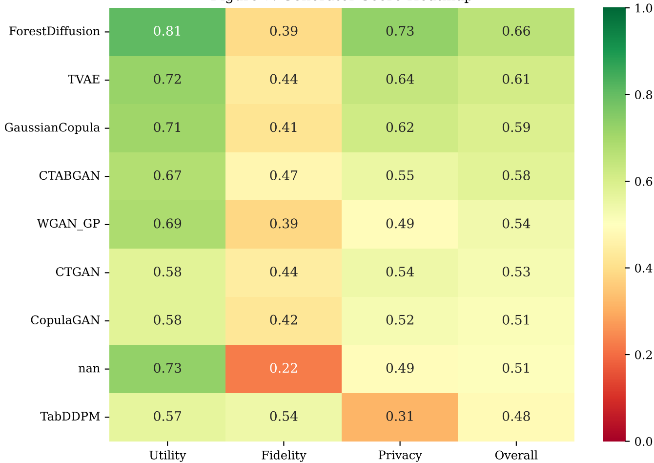
Figure 7: Generator Score Heatmap
